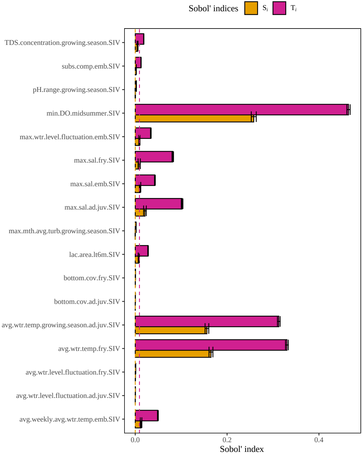
Figure 3. Results of a sensitivity analysis for the largemouthbassLacS model based on the original author-specified model outlined in Stuber et al. (1982). Dashed lines represent baseline numerical approximation error for S_i and T_i ( i.e. , dummy variables).
