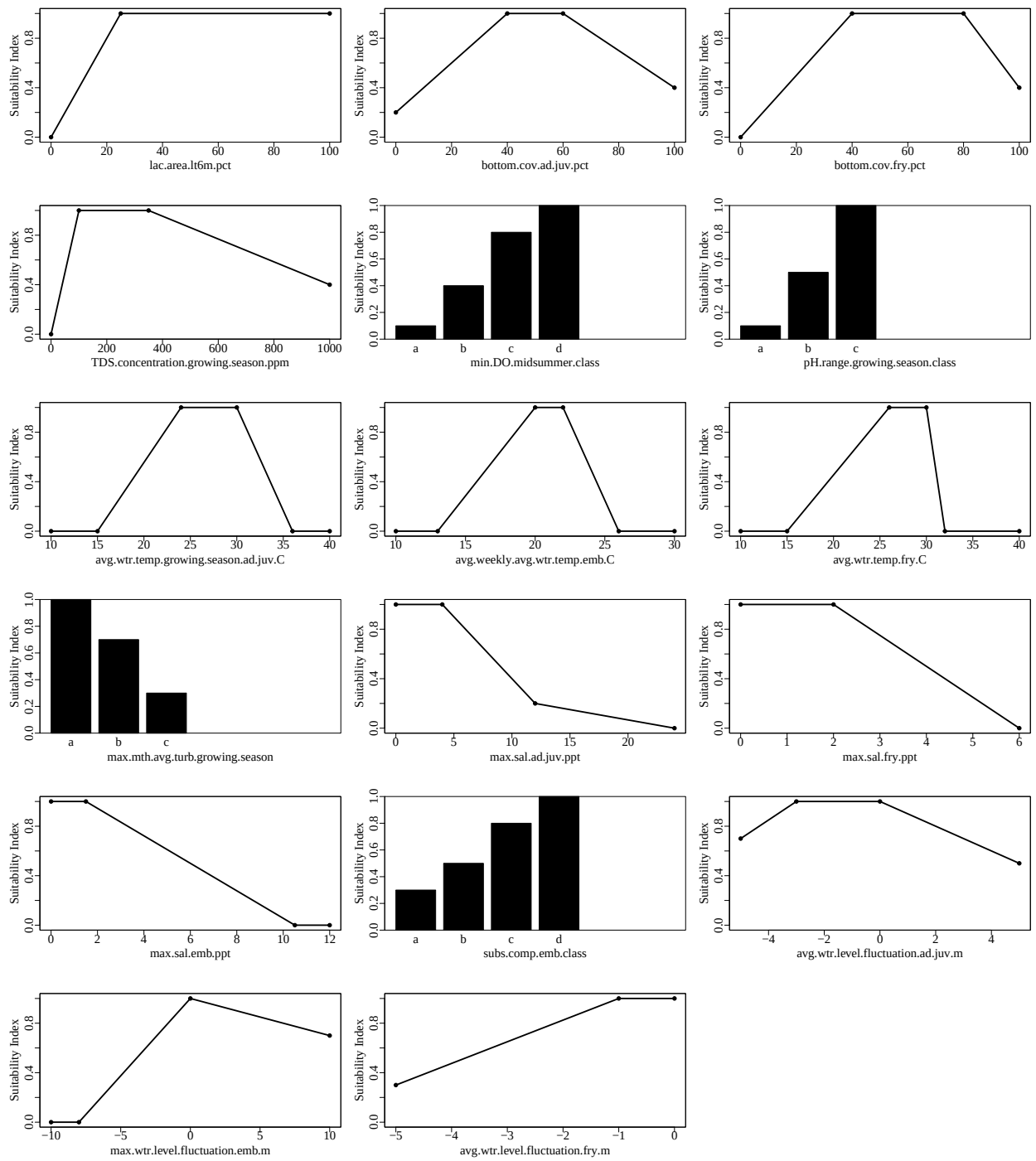
Figure 1. Suitability index graphs for variables included in the largemouthbassLacS model in ecores.
