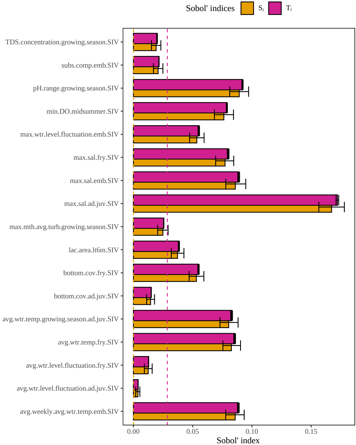
Figure 5. Results of a sensitivity analysis for the largemouthbassLacS model based on a geometric mean structure. Dashed lines represent baseline numerical approximation error for S_i and T_i ( i.e. , dummy variables).
